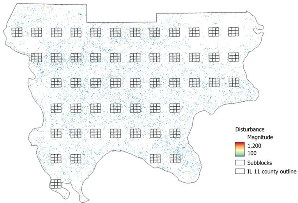
Figure A3.1. Forest associated disturbance between 2016-2021 from LandTrendR algorithm filtered by yearly forest cover in LCMS Land Use.
