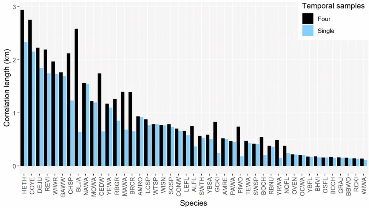
Fig A4.1. Correlation length (km) for species for which we fit species distribution models. Associated species 4-letter codes, common names and genus species are reported in Appendix 2, Table A2.1.
