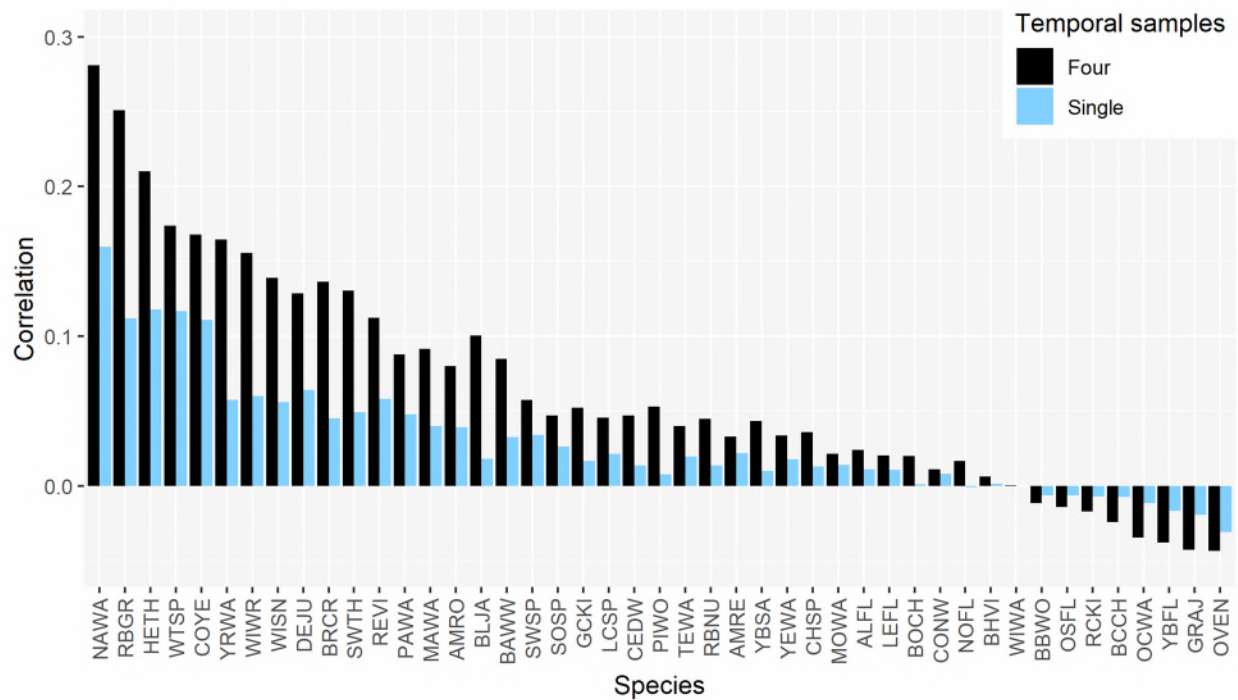
Fig A4.2. Spatial correlation between adjacent secondary sampling units for species for which we fit species distribution models. Associated species 4-letter codes, common names and genus species are reported in Appendix 2, Table A2.1.
