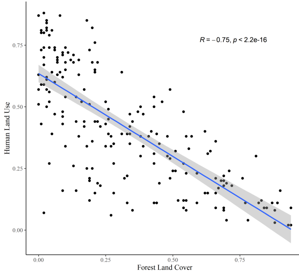
Figure A1.6. Correlation between proportion human land use and proportion forest cover for sites surveyed in the upland coastal zone of the Great Lakes ( n = 199 sites).
