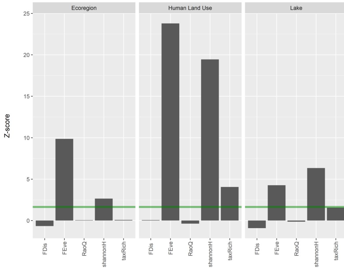
Figure A1.4. Plot of z-scores for independent contributions (I) of the human land use gradient, ecoregion, and lake to measures of functional and taxonomic diversity based on 100 randomizations using hier.part package in R. The green horizontal line represents the upper 95% confidence value for the Z-scores (1.65) and is used as an indication of statistical significance.
