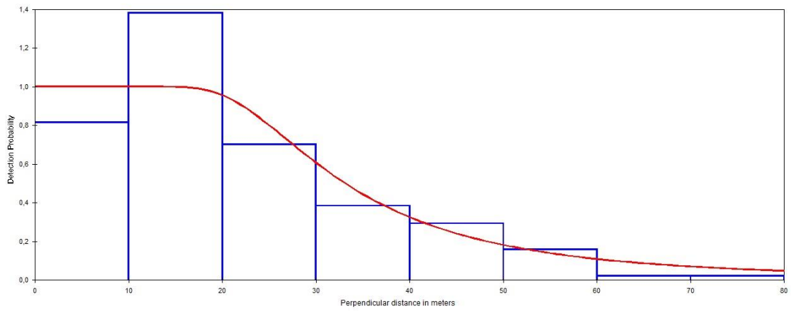
Figure A1.3. Detection probabilities of the Black-cheeked Gnatcatcher at different perpendicular distances, and adjustment of the Hazard-Rate Cosine detection function.
