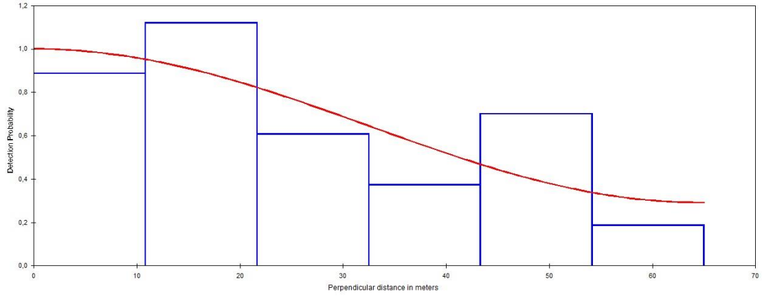
Figure A1.1. Detection probabilities of the Pernambuco Fire-eye at different perpendicular distances, and adjustment of the Uniform Cosine detection function.
