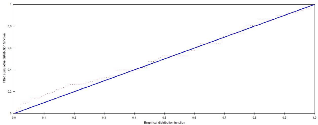
Figure A1.4. Quantile-quantile plot (Q-q plot) generated for the Black-cheeked Gnatcatcher evidencing the fit of the Hazard-Rate Cosine detection function to the data.
