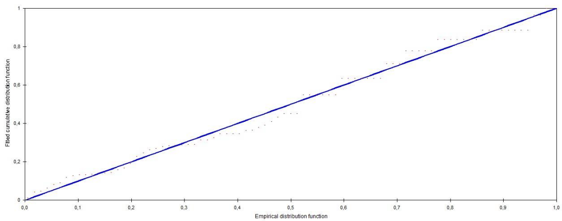
Figure A1.2 Quantile-quantile plot (Q-q plot) generated for the Pernambuco Fire-eye evidencing the fit of the Uniform Cosine detection function to the data.
