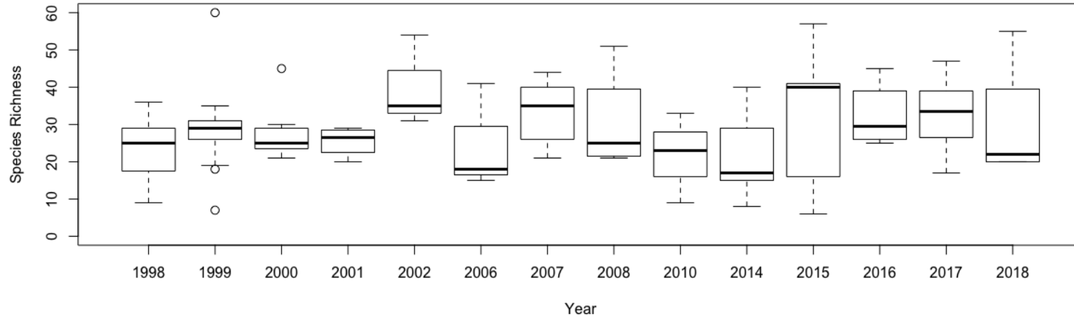
Appendix 5. Boxplot of species richness for years with the highest representation on data.
