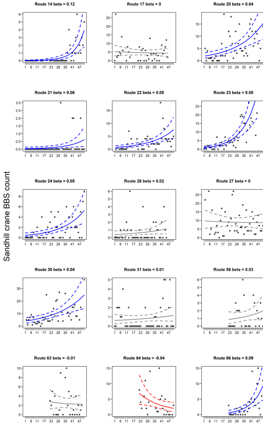
Fig. A3.1. Route-specific raw counts (black circles) and trend lines (blue, red, and gray lines indicate significantly positive, significantly negative, and no trends, respectively) for 42 Breeding Bird Survey routes for which data were available from 1966 through 2016. Trends are estimated from the model described in Appendix 2.
