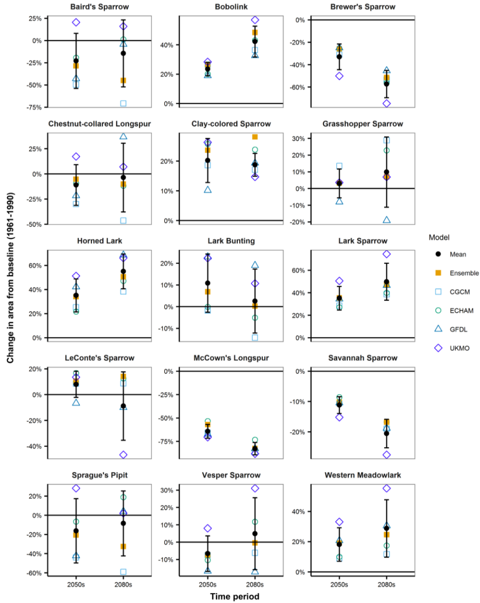
Figure A5.1. Projected changes in core suitable climate area in North America from the historical baseline (1961-1990) for the 2050s (2041-2070) and the 2080s (2071-2100). The mean change ( \pm 95% CI; black circles) is determined from the four unique GCMs (CCCMA CGCM3.1; MPI ECHAM5/MPI-OM; GFDL CM2.1; UKMO-HadGEM1; open symbols). Changes in areas projected using ensemble climate data (yellow squares) correspond to the maps in Figure A3.1.
